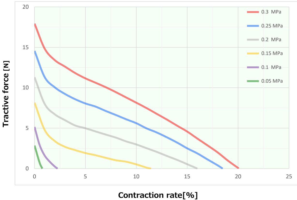
[PMJ20series] Relationship between tractive force and contraction rate (reference data)
