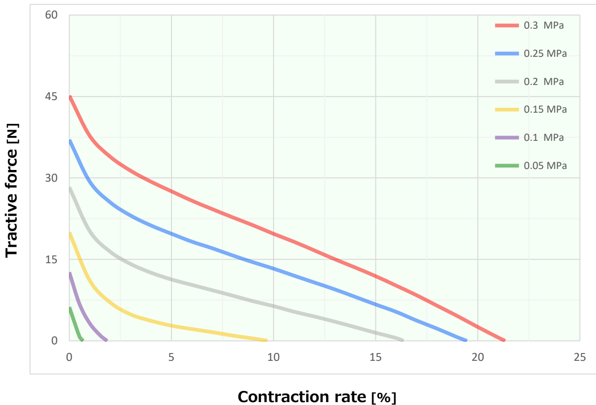
[PMJ40series] Relationship between tractive force and contraction rate (reference data)
